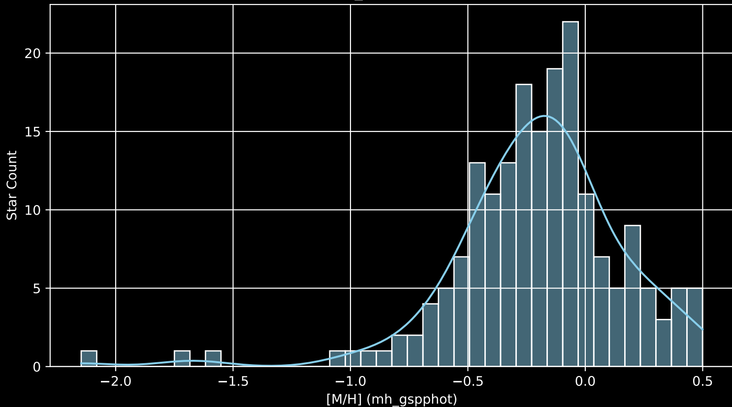
APOGEE DR17 Field: [154+59_MGA [M/H] (mh_gspphot) (n= 188)
