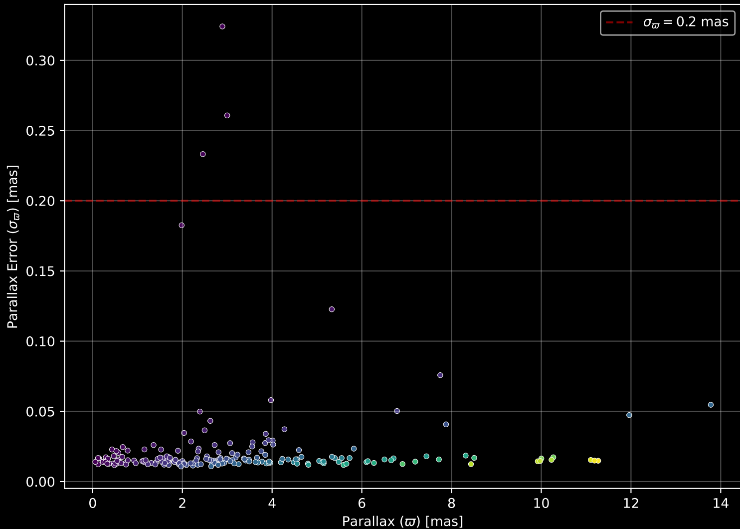
APOGEE DR17 Field: [154+59_MGA] Parallax Quality (n= 191)
