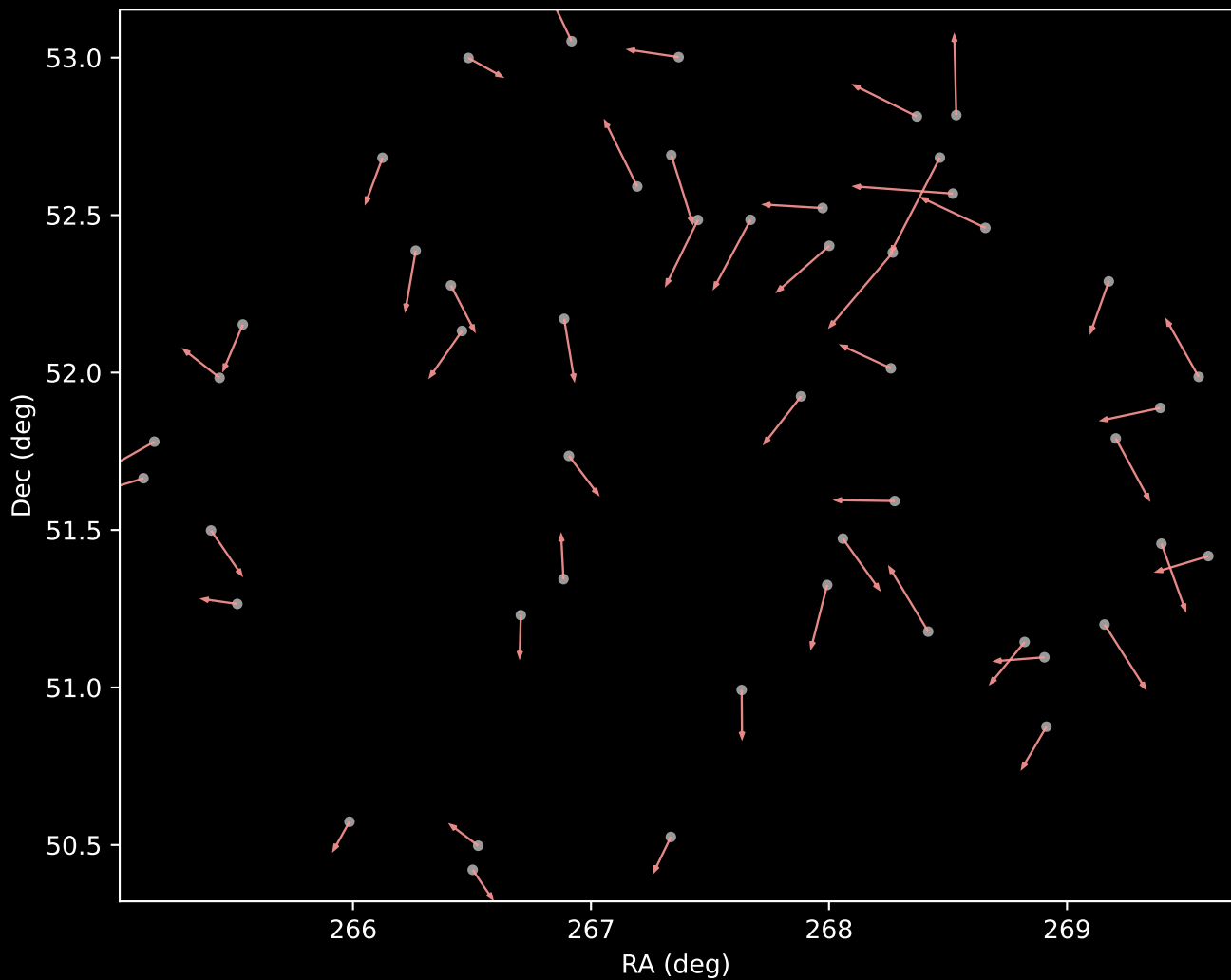
APOGEE DR17 Cluster 7 Proper Motion Vectors (n=50)
