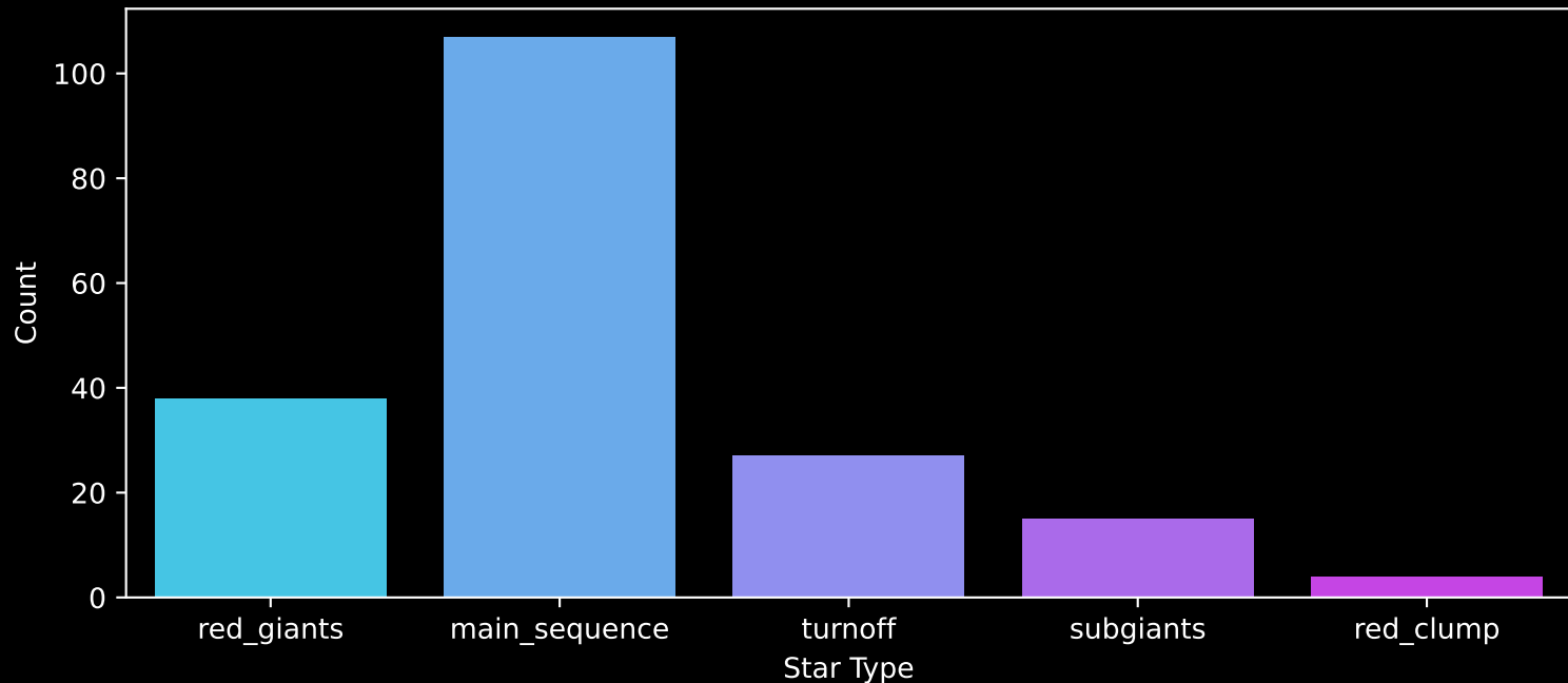
APOGEE DR17 Field: [154+59_MGA] Count plot of Star Type
