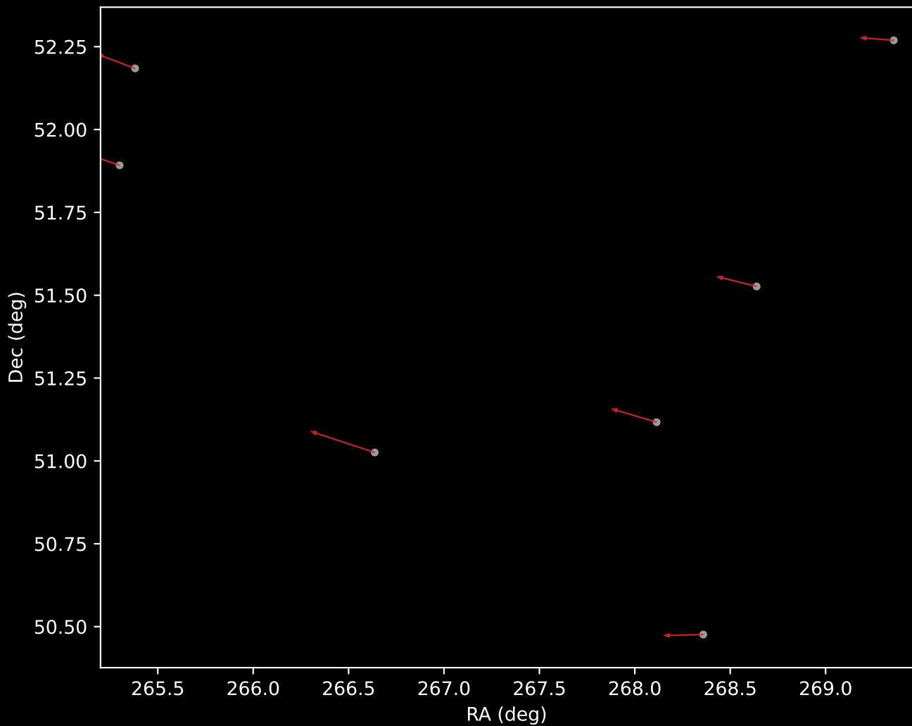
APOGEE DR17 Cluster 6 Proper Motion Vectors (n=7)
