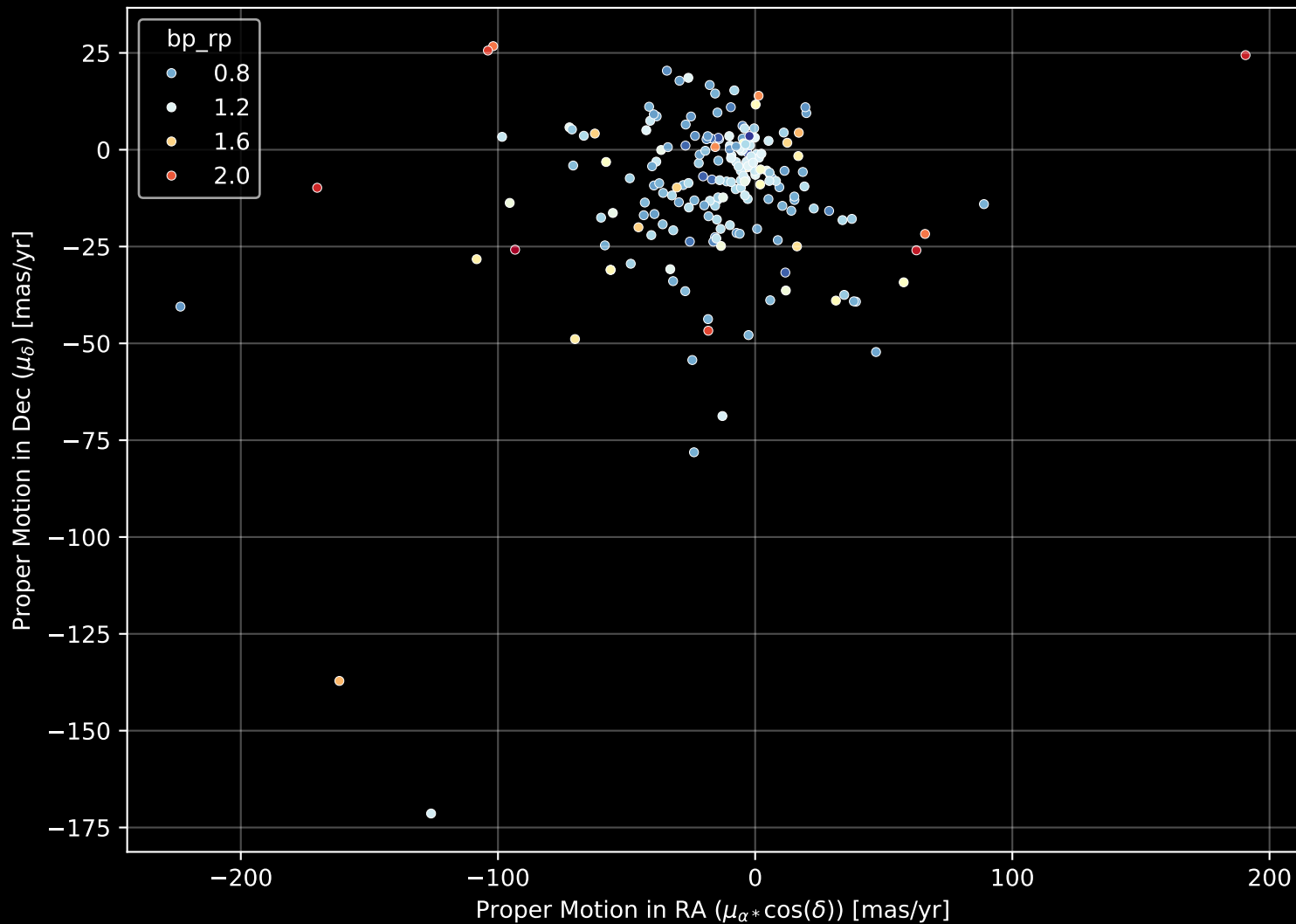
APOGEE DR17 Field: [154+59_MGA] Proper Motion Diagram (n= 191)
