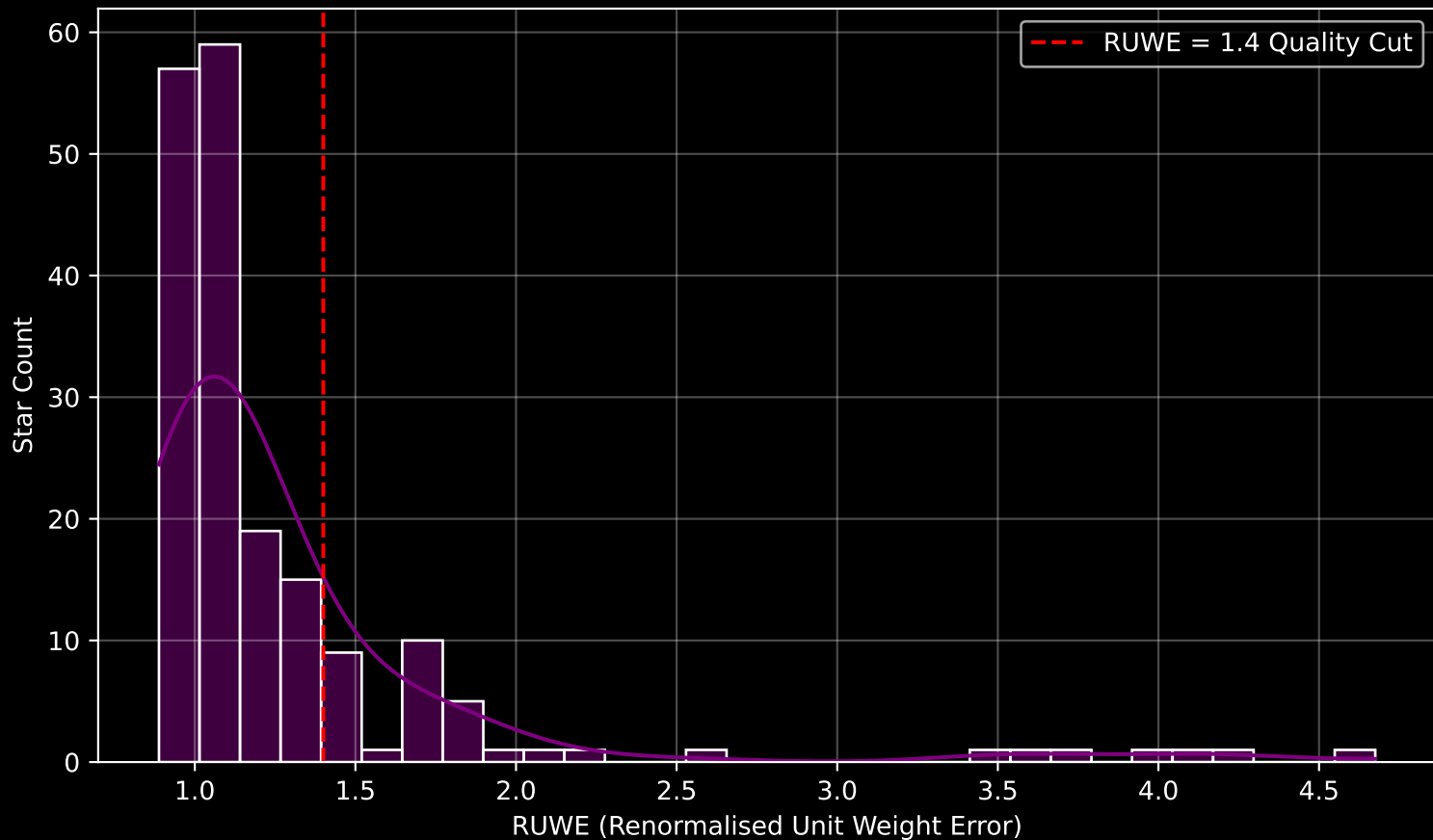
GAPOGEE DR17 Field [154+59_MGA] RUWE Distribution (n= 186)
