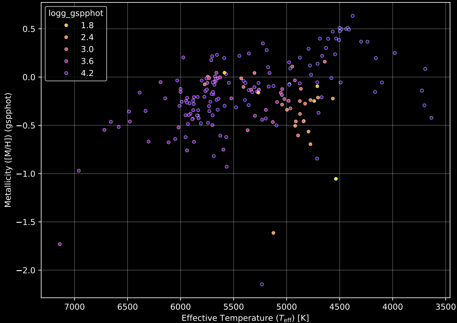
APOGEE DR17 Field: [154+59_MGA] Stellar Population Parameters (n= 191)
